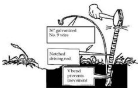
Fig. 32. Driving the snare wire
