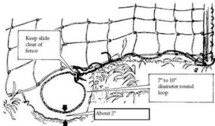
Fig. 35. Snare set for woven wire
