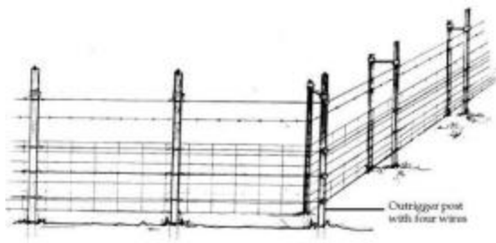
Fig. 5. Existing woven-wire livestock fence modified with electrified wire.
