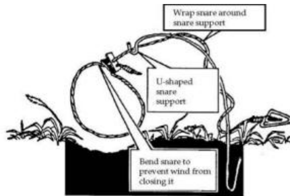
Fig. 33. Setting the snare
